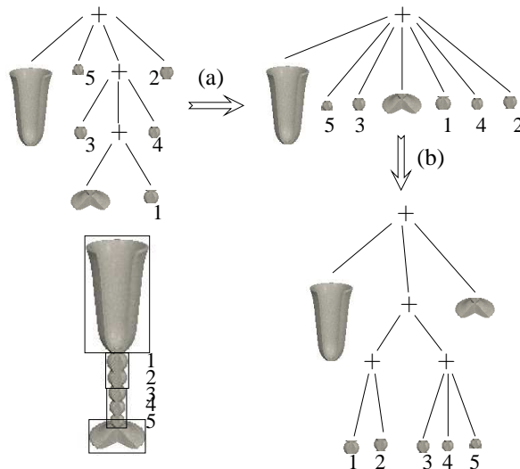
Figure 14: Optimization of the scene graph: merge the nodes of the same type to reduce the depth and balance the tree to create an optimized bounding boxes hierarchy.
