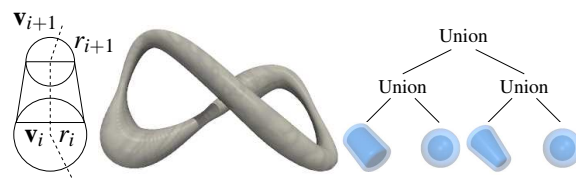
Figure 5: A LOD - generalized cylinder primitive and its corresponding BlobTree representation.
